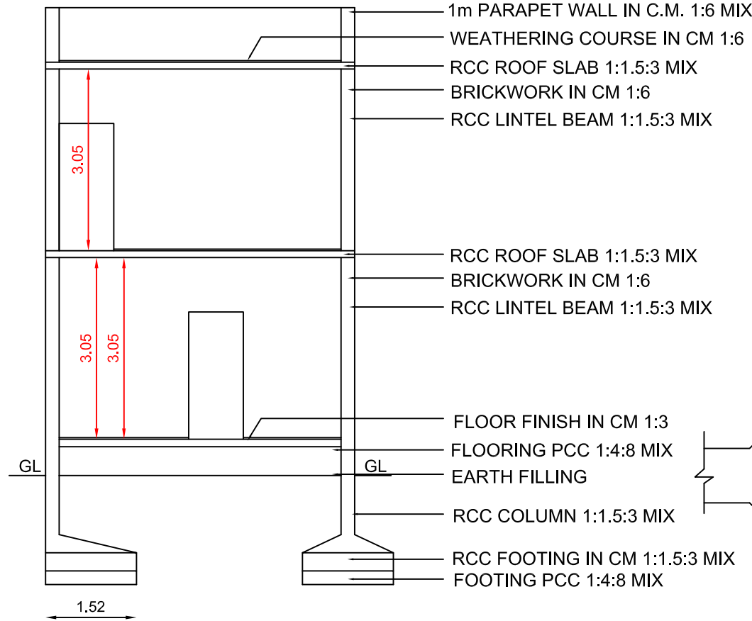
CROSS SECTION ON XY
