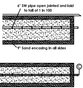
TIC TANK (NTS)
