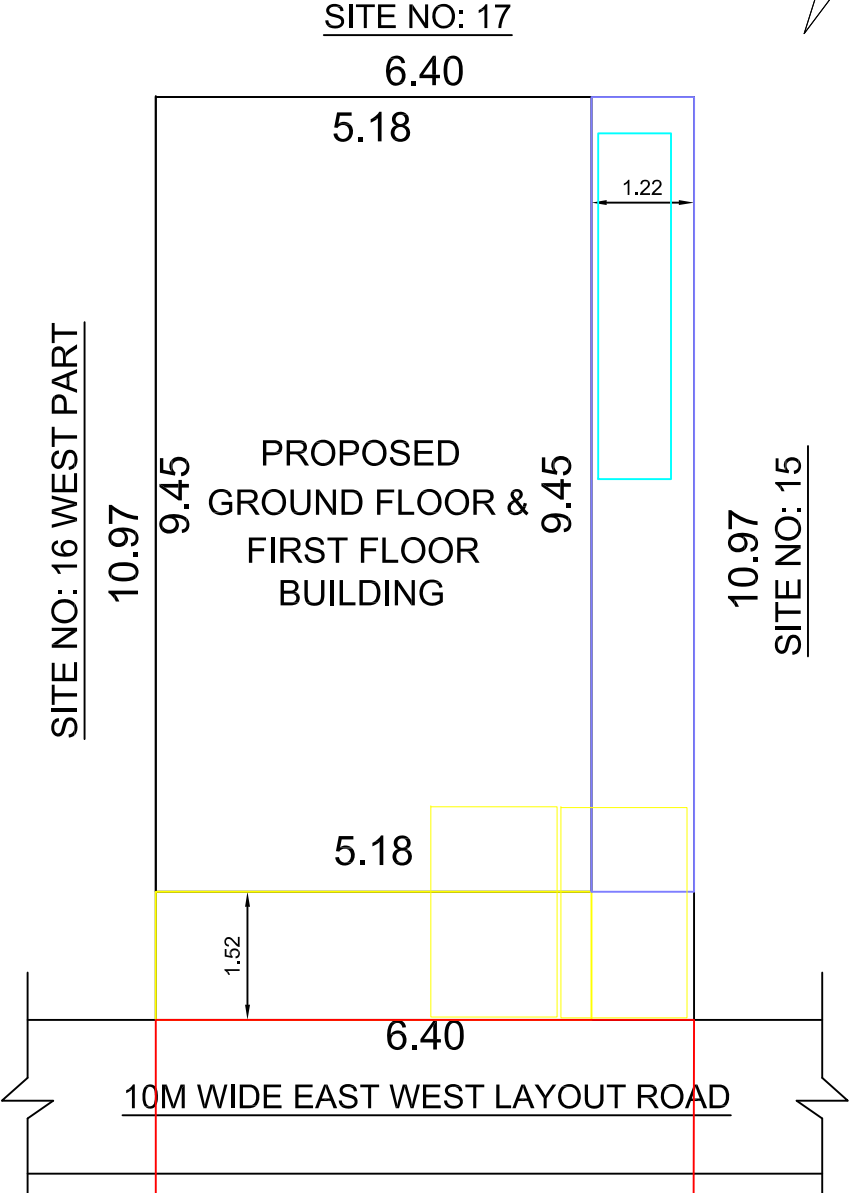
SITE PLAN
