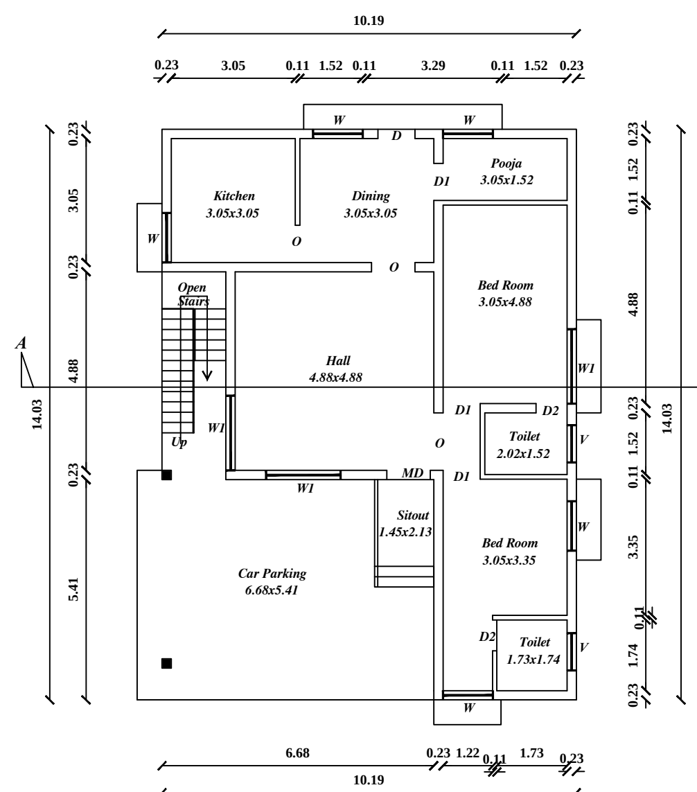
Ground Floor Plan (Exg.) (SCALE: 1" = 8' 0")
