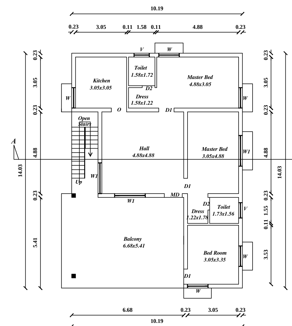
First Floor Plan (Pro.) (SCALE: 1" = 8' 0")
