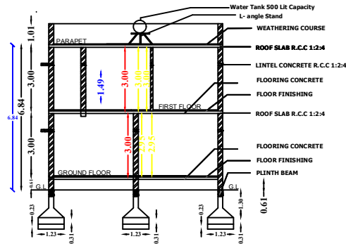
SECTION
