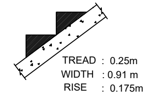
STAIRCASE DETAIL:
