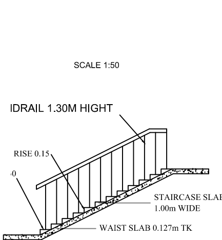
STAIRCASE DETAILS
