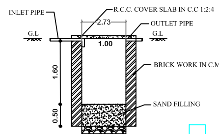
SECTIONAL DETAILS
