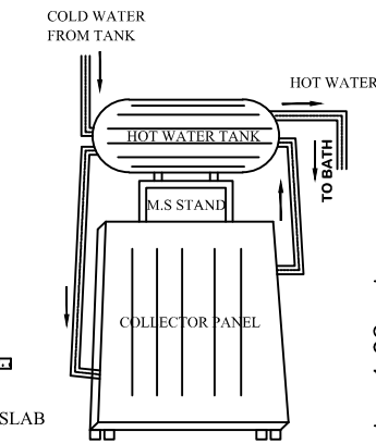
SOLAR WATER HEATER SYSTEM
