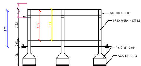
SECTION AB
