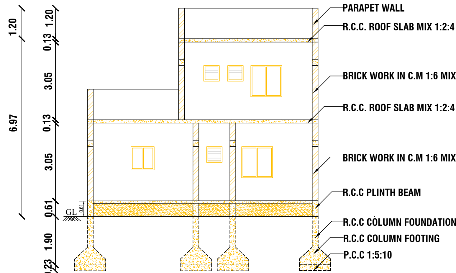
CROSS SECTION AT A-A
