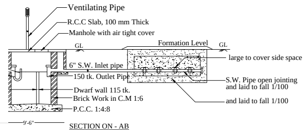
C TANK WITH DISPERSION TRENCH (250 Gls.)
