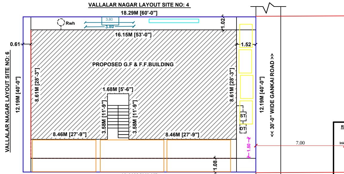
SITE PLAN
