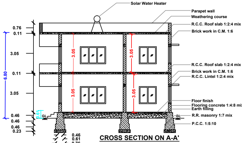
CROSS SECTION ON A-A'
