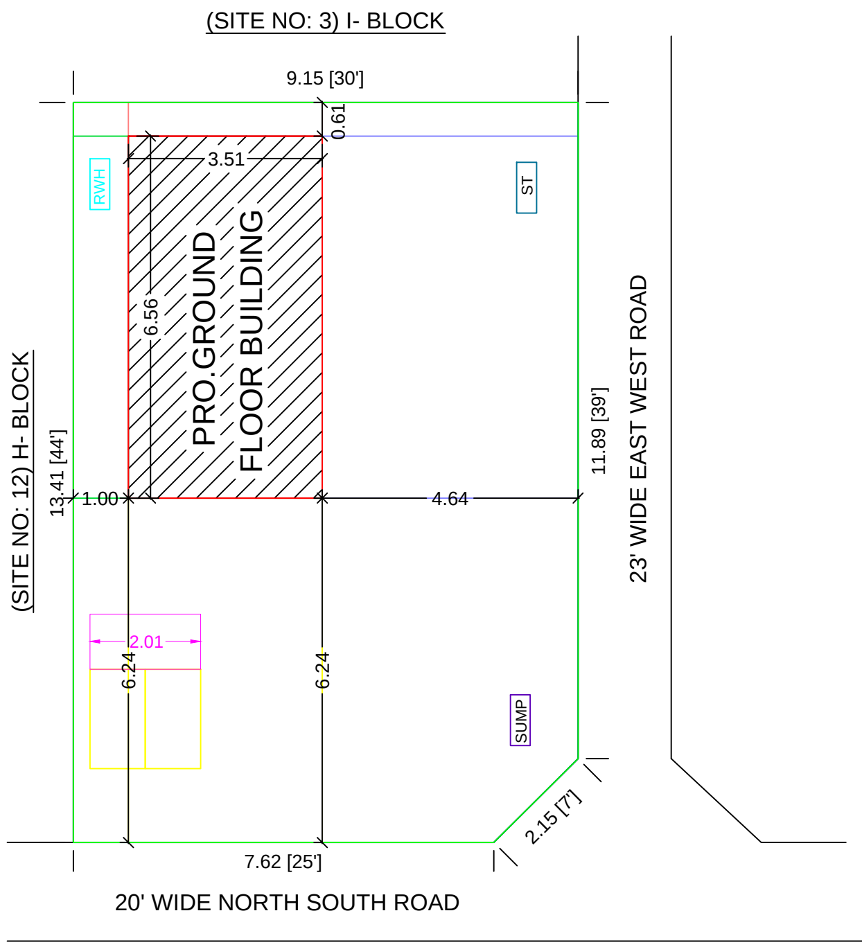
SITE PLAN
