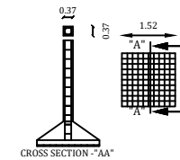
COLUMN DETAILS :-
