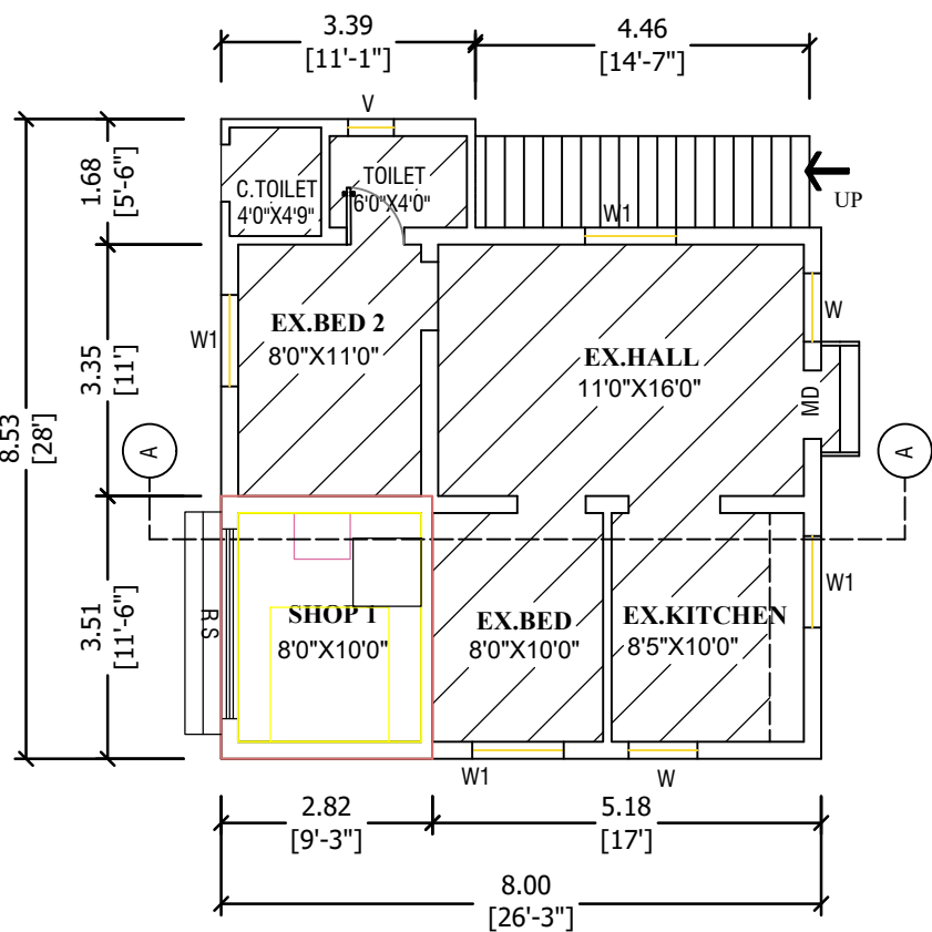
PROPOSED ADD.GROUND FLOOR
