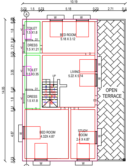
PROPOSED FIRST FLOOR BUILDING
