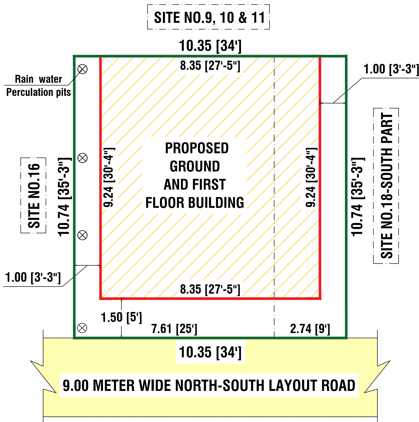
SITE PLAN
