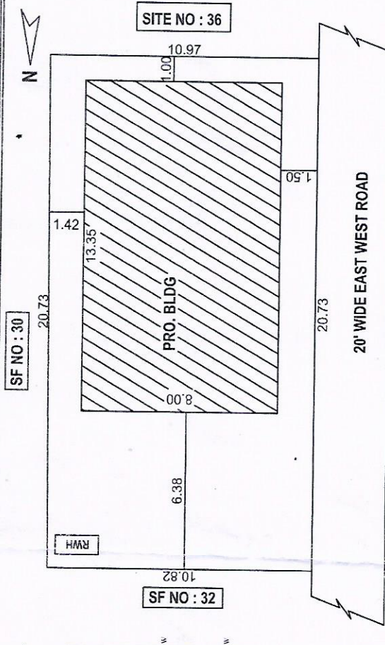
SITE PLAN
