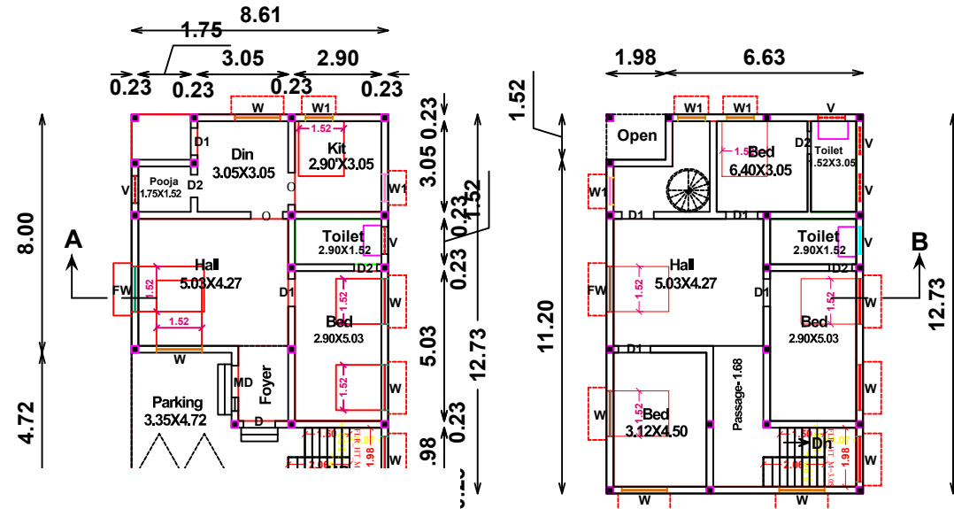
F.FLOOR PLAN
