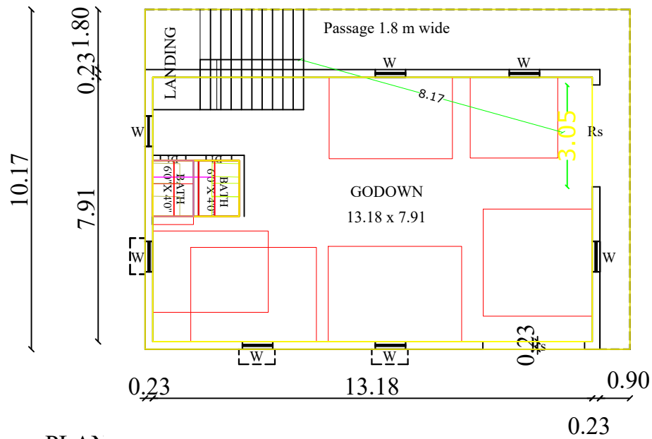
PLAN
