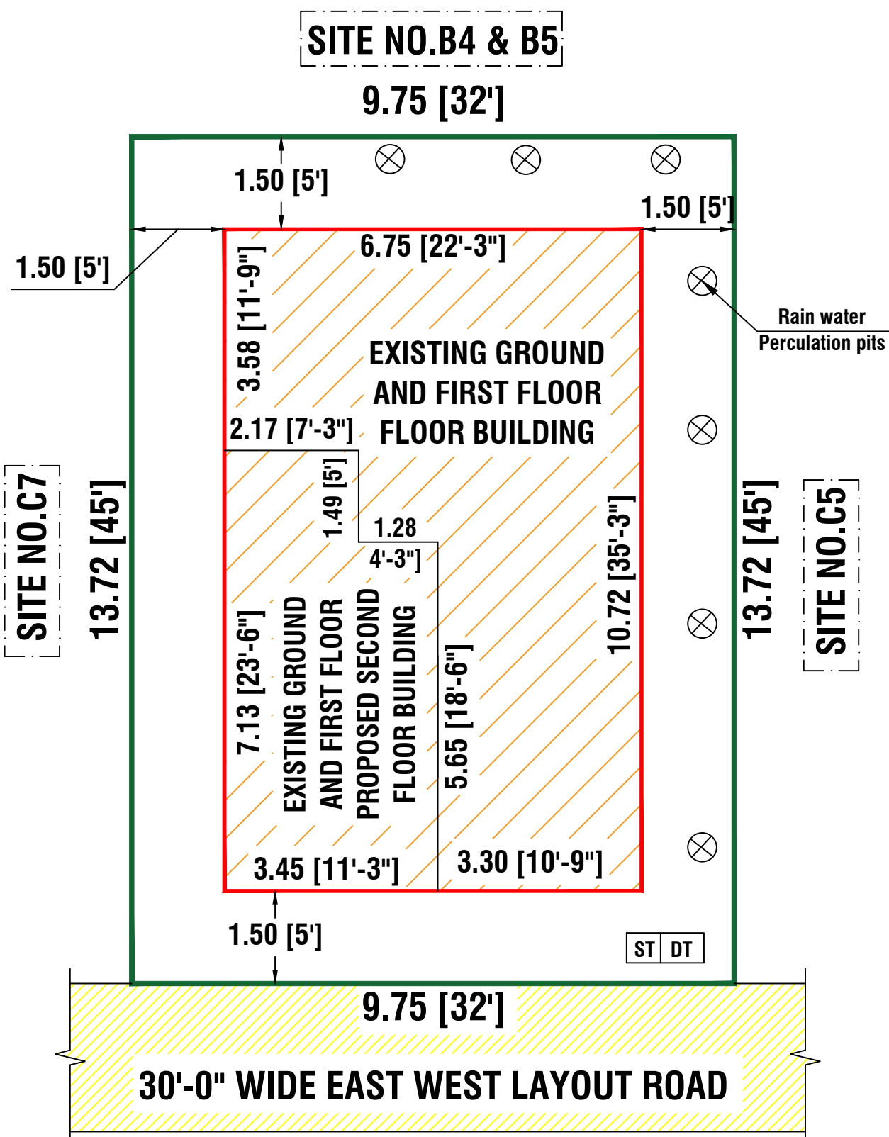
SITE PLAN
