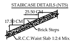
STAIRCASE DETAILS (NTS)
