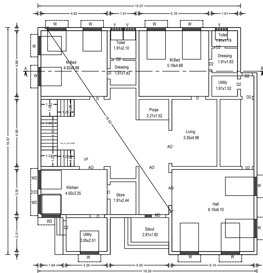
Plan Scale 1:100 Ground floor
