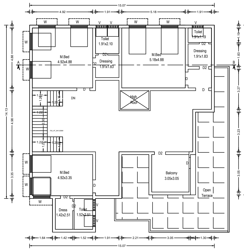
Plan Scale 1:100 First floor
