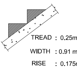
STAIRCASE DETAIL:
