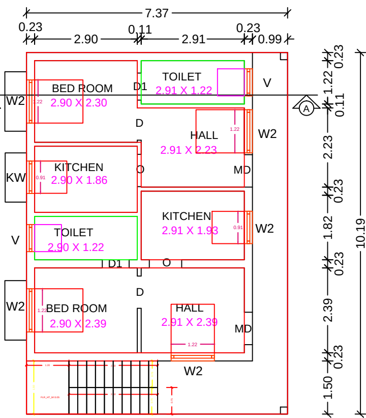
EXT.FIRST FLOOR PLAN
