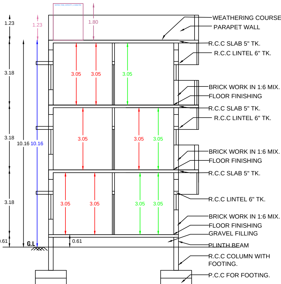
CROSS SECTION A-A
