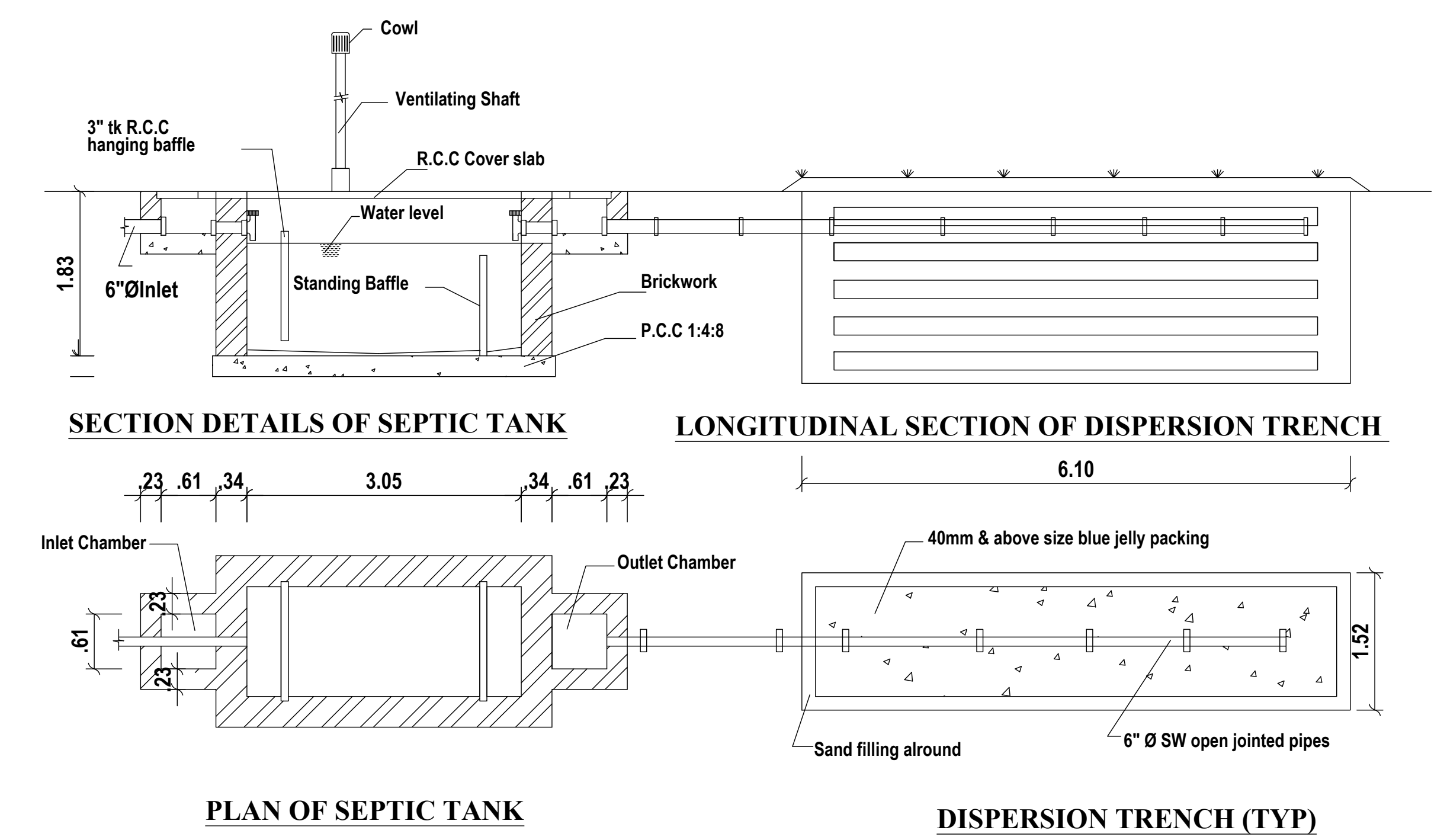
DETAILS OF SEPTIC TANK - 250 GALLONS & DISPERSION TRENCH
