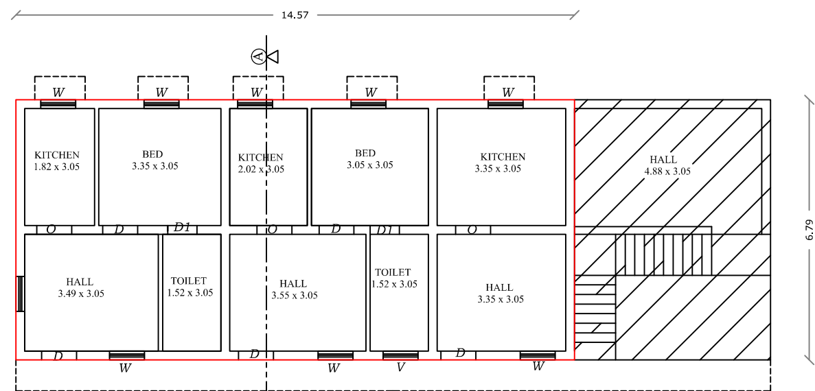
EXISTING & PROPOSED FIRST FLOOR PLAN
