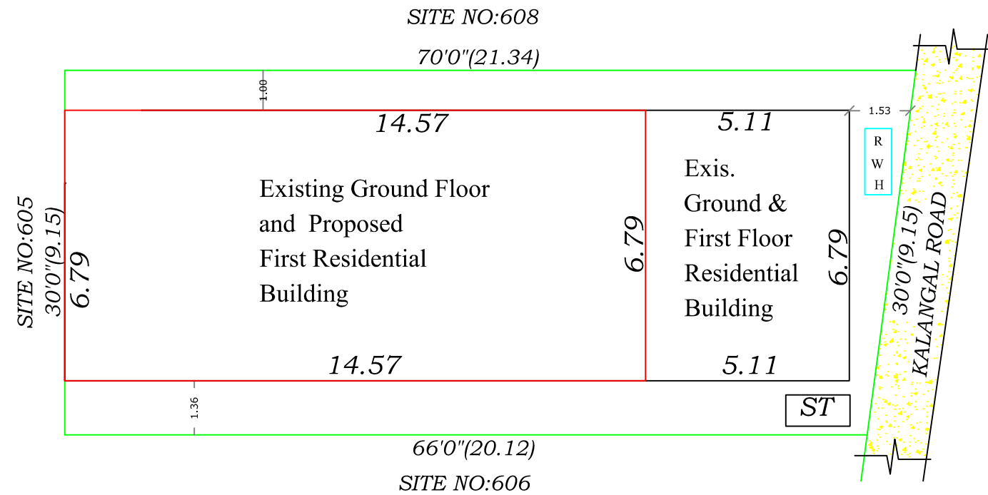
SITE PLAN
