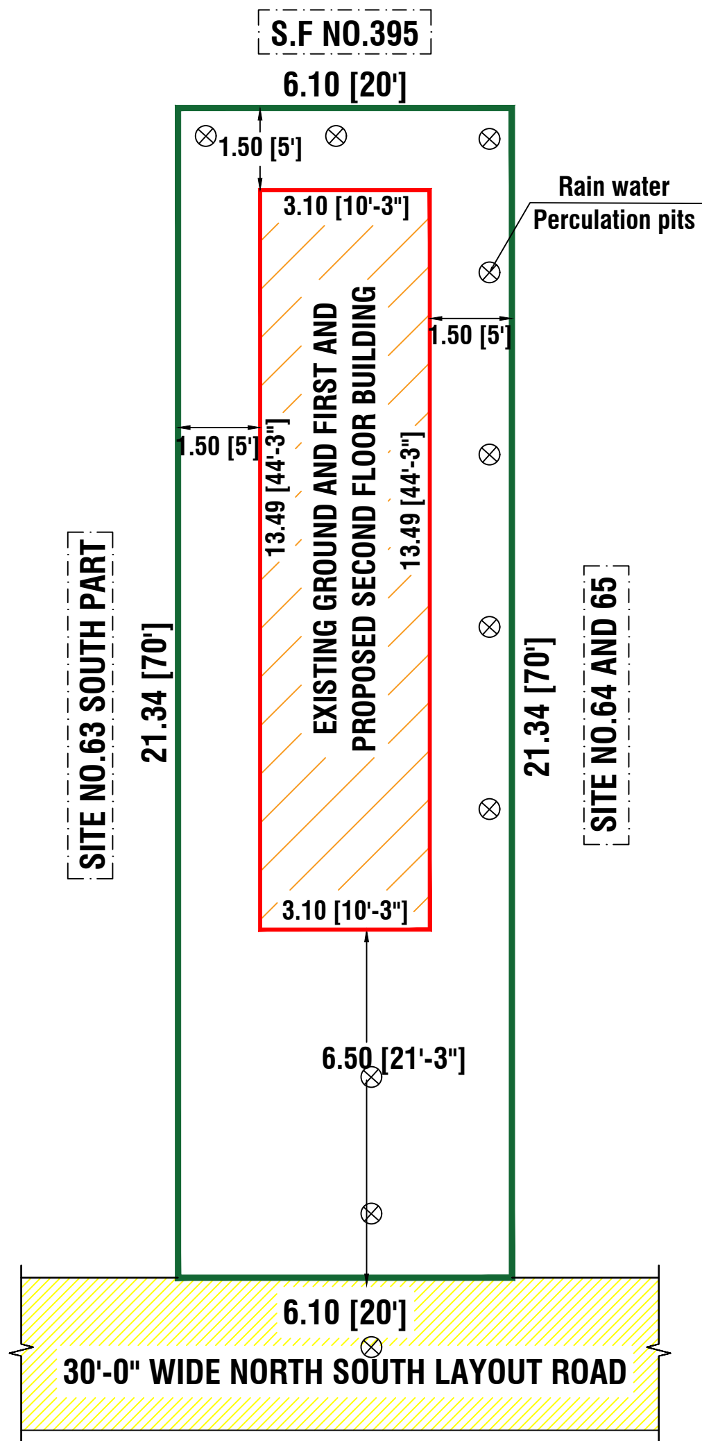
SITE PLAN
