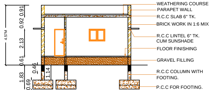
CROSS SECTION AT A-A
