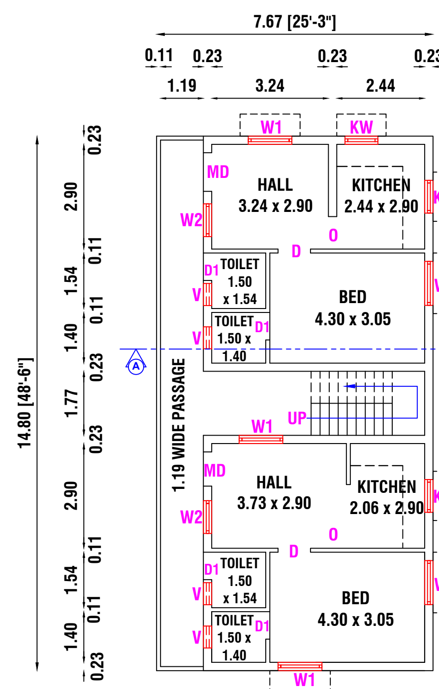
SCOND FLOOR PLAN
