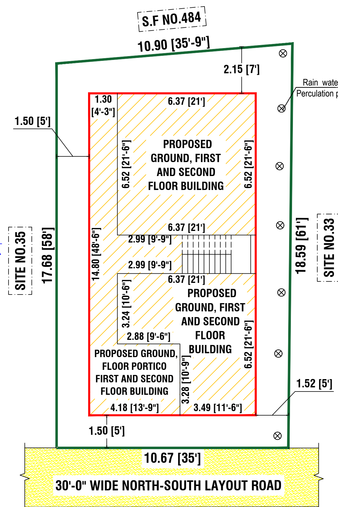
SITE PLAN
