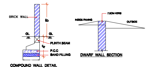
COMPOUND WALL DETAIL DWARF WALL SECTION
