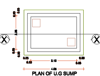
PLAN OF U.G SUMP
