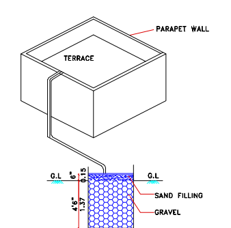
COLLECTION SUMP FOR HARVESTING FOR TERRACE
