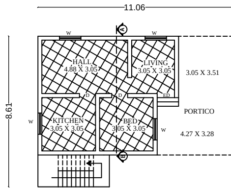
EXG. & PRO. ADD GROUND FLOOR PLAN
