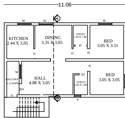
PRO. ADD FIRST FLOOR PLAN
