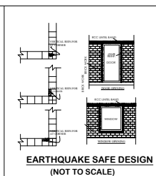
SEISMIC REINFORCEMENT DETAILS
