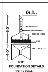
FOUNDATION DETAILS (NOT TO SCALE)
