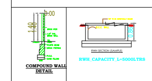
DETAIL
