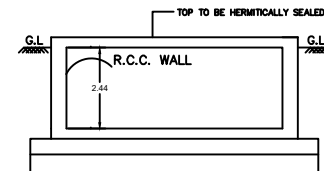
RWH_CAPACITY_L = 2000LTRS
