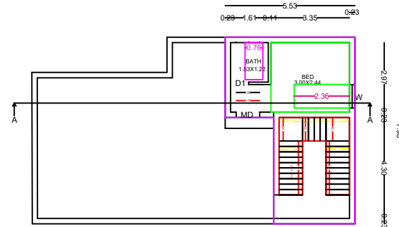
EXISTING AND ADDITIONAL PROPOSED FIRST FLOOR PLAN
