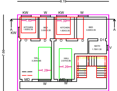
3 FIRST FLOOR
