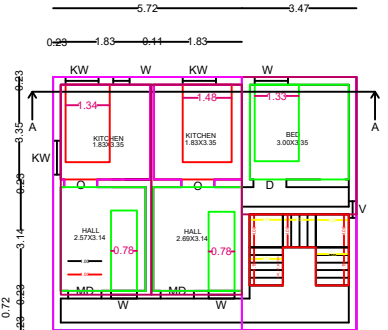
EXISTING AND ADDITIONAL PROPOSED SECOND FLOOR PLAN
