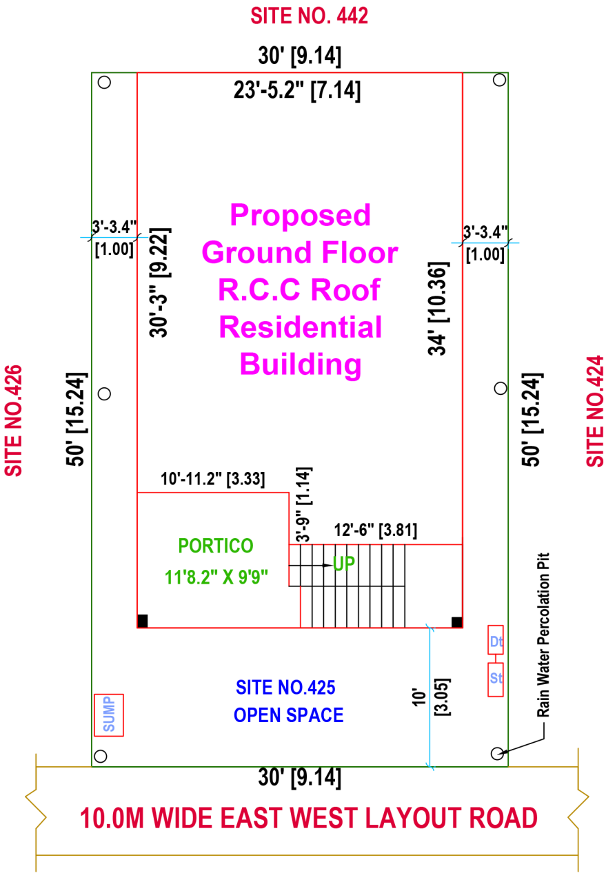
SITE PLAN
