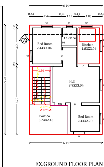
EX.GROUND FLOOR PLAN
