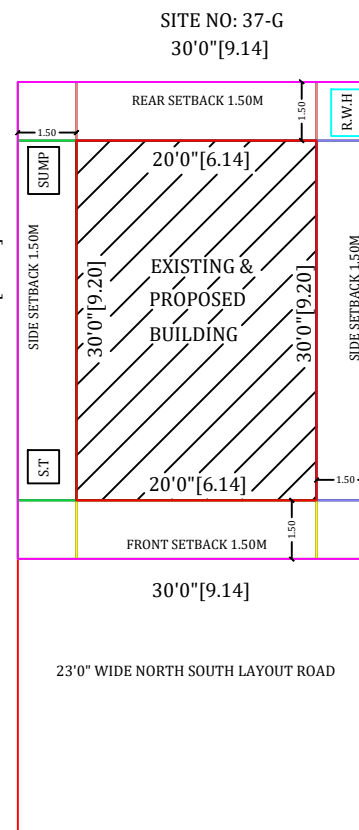
SITE PLAN
