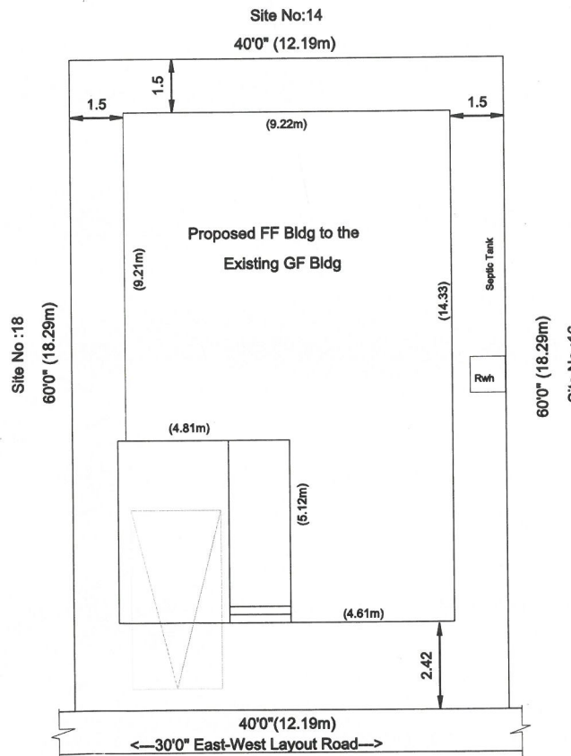
SITE PLAN
