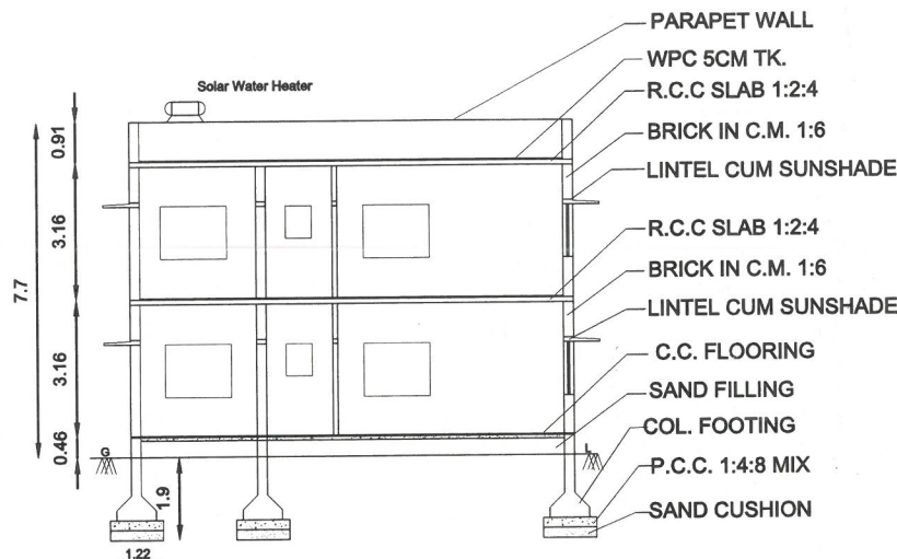
SECTION "AB"
