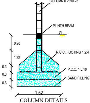
COLUMN DETAILS
