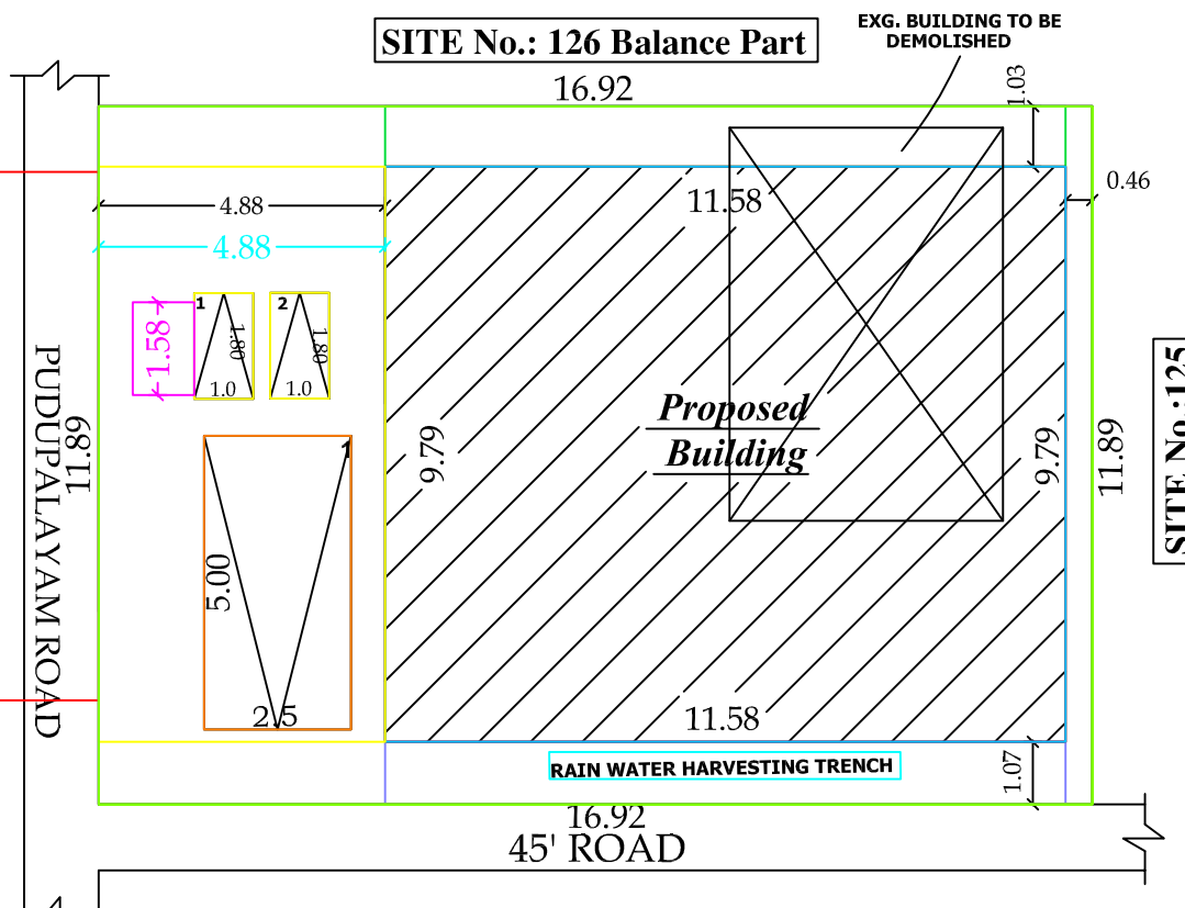
SITE PLAN
