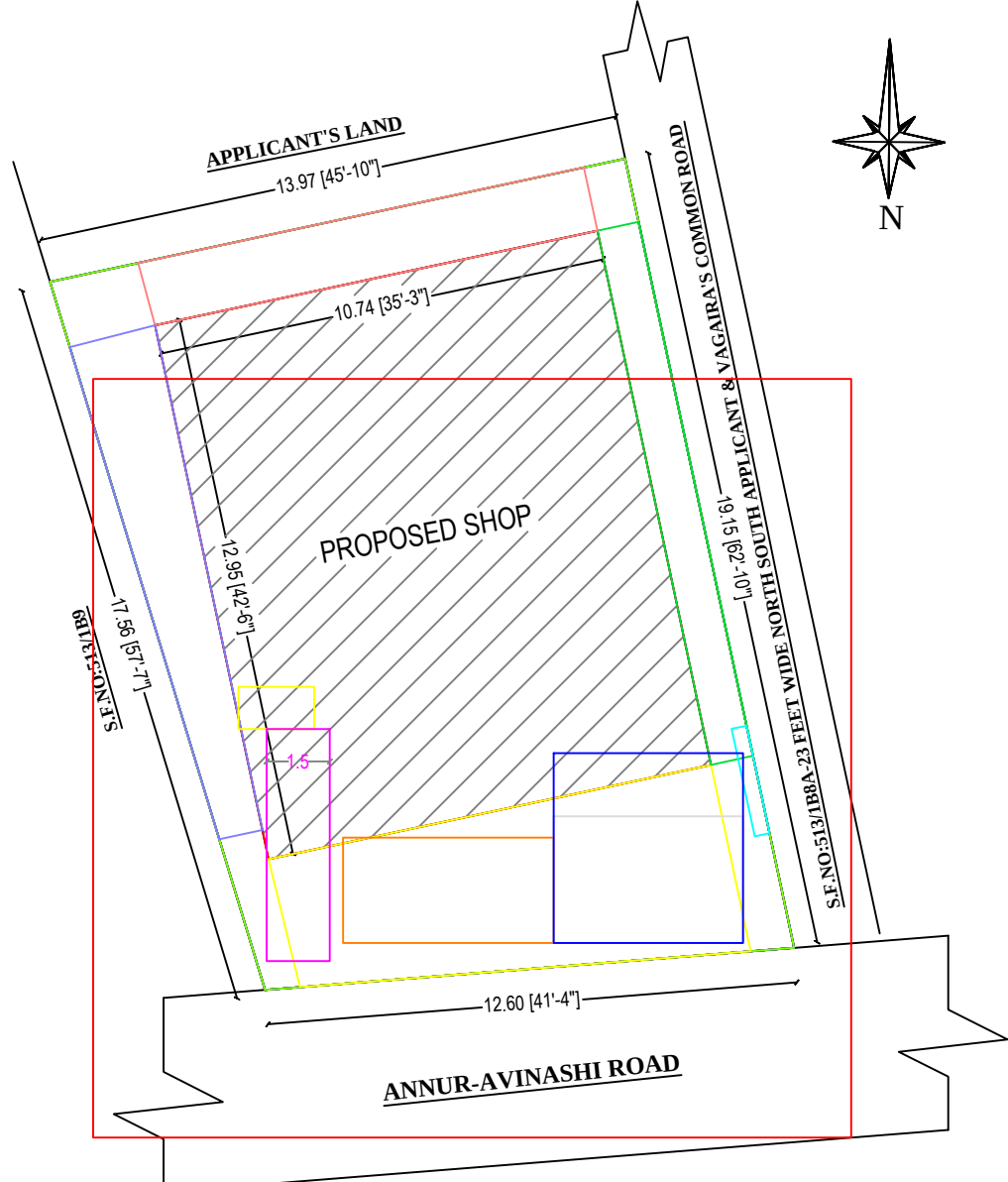
SUPER IMPOSED PLAN
