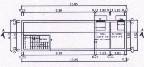
PRO. SECOND FLOOR PLAN
