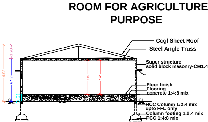
SECTION ELEVATION
