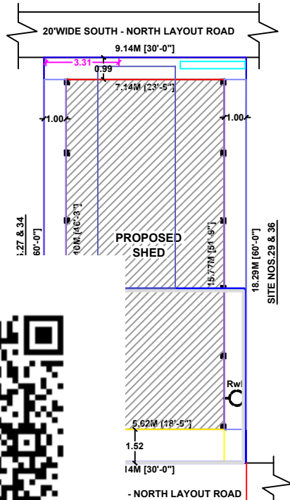
Site Plan
