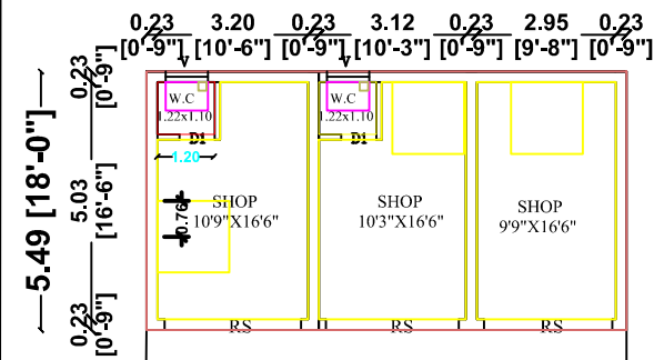
PROPOSED PLAN
