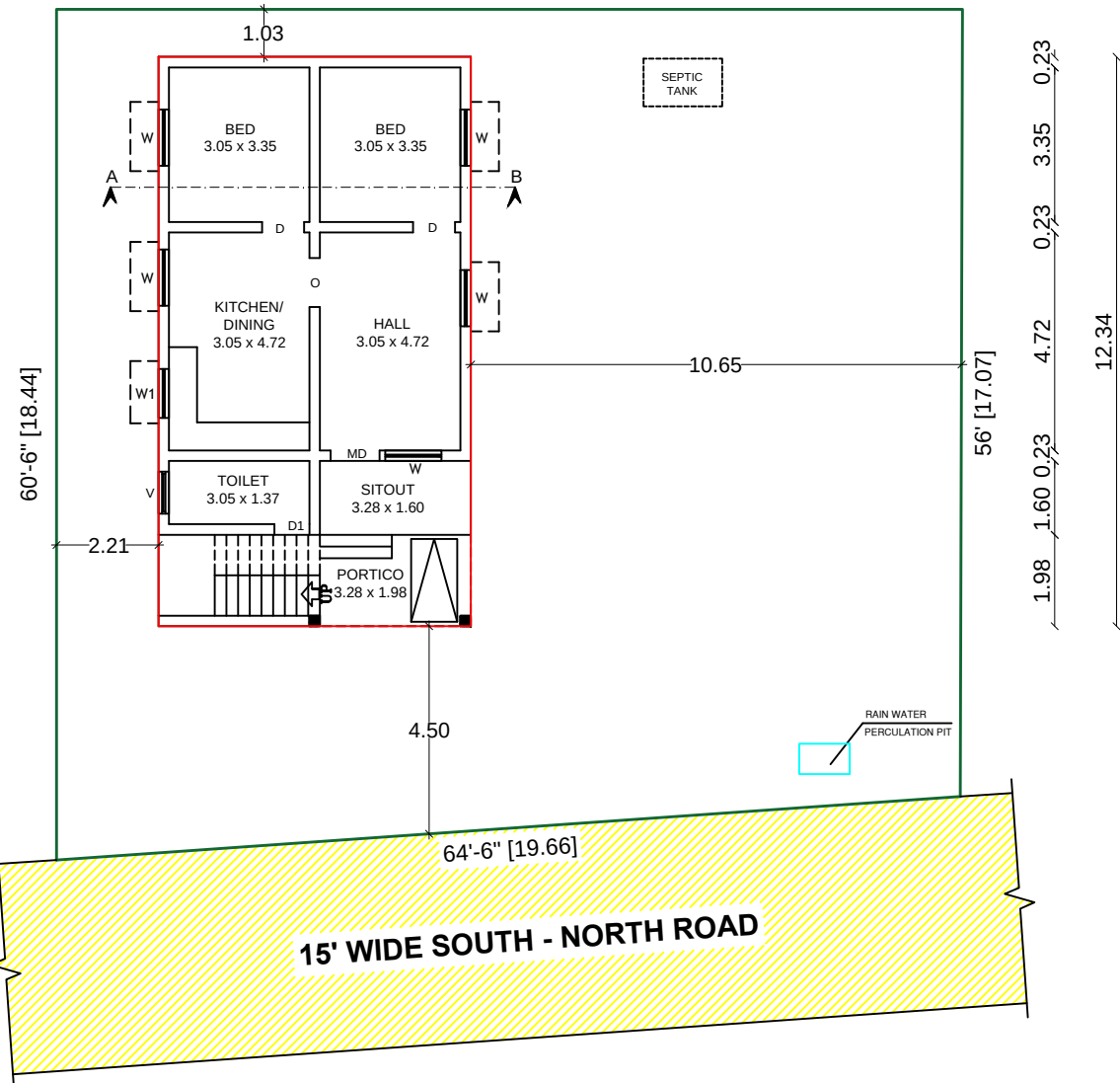
SITE CUM GROUND FLOOR PLAN
