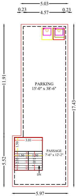
STILT FLOOR PLAN
