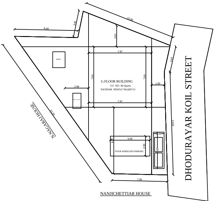
SITE PLAN
