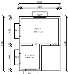
ROUND FLOOR PLAN
