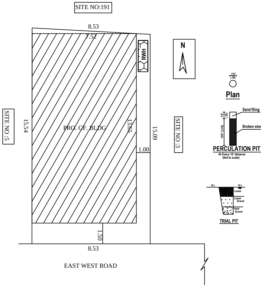
SITE PLAN
