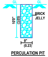
PERCOLATION PIT
