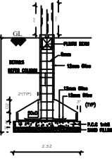
FOUNDATION DETAILS
