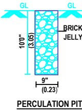
PERCOLATION PIT
