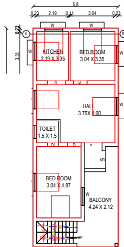
PROPOSED ADDI. FIRST FLOOR BUILDING
