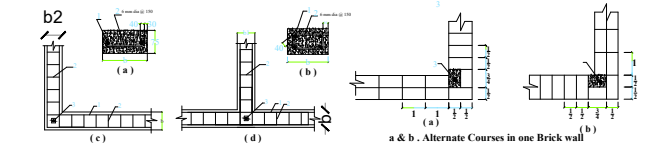
Figure - 1 :Essential Internal Elements in Buildings for Earthquake Safety.
