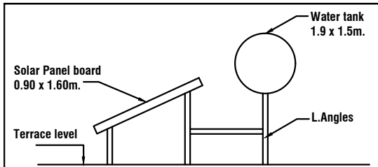
CROSS SECTION OF SOLAR WATER HEATING SYSTEM
