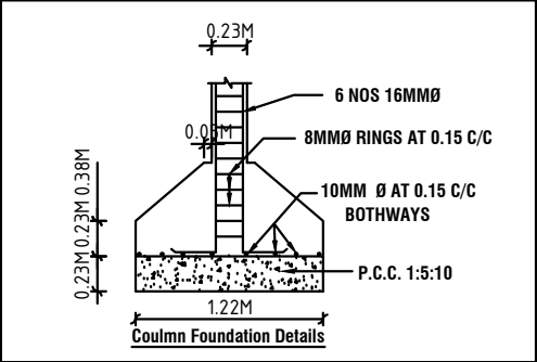
Column Foundation Details
