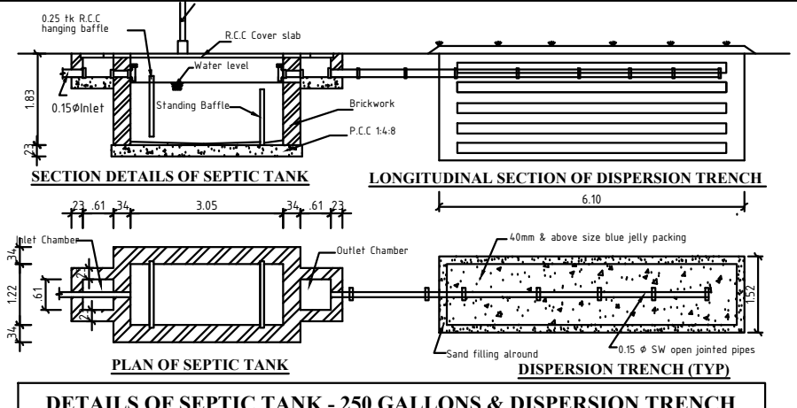
DETAILS OF SEPTIC TANK - 250 GALLONS & DISPERSION TRENCH
